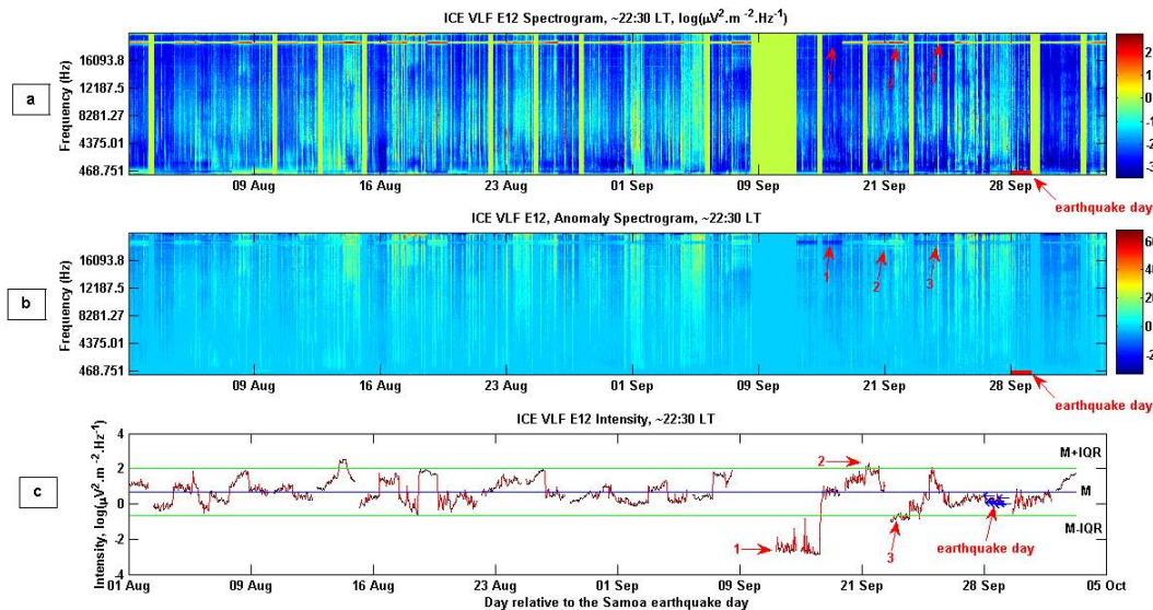
Fig. 2. Results of the DEMETER data analysis concerning the Samoa earthquake (29 September 2009) from 1 August to 5 October 2009 at ~22:30 LT. Due to the operation of satellite in safe mode a time gap is observed from 7 to 15 September 2009. The earthquake day is represented by a red tick below the X-axis. (a) ICE VLF spectrogram of the E12 electric component. The intensity of the spectrogram is color-coded according to the scale on the right. (b) Detected anomaly in the ICE VLF spectrogram of the E12 electric component. The anomaly is color-coded according to the scale on the right. (c) Intensity of ICE VLF spectrogram of the E12 electric component around the virtual NPM transmitter frequency (see text for explanation). For this panel the green horizontal lines indicate the higher and lower bounds ( M \pm IQR ). The blue horizontal line indicates the median value ( M ). In all panels, the X-axis represents days relative to the occurrence of the Samoa earthquake.
