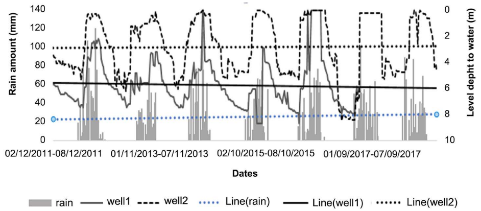
Figure 3. Rainfall status and fluctuation of water table in wells 1 & 2 in Basbédo.
