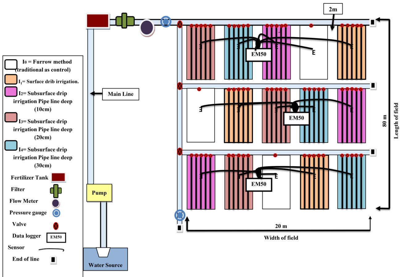
Figure 4. Experimental Layout.
