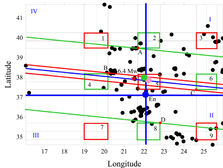
Figure 19. Procedure applied to the 08/06/2008 Greece earthquake seismic sequence. The map shows the hazard bands. The solid blue colored circle (En) indicates the last recorded earthquake. The quadrants are indicated with the letters I, II, III and IV in blue color. The red star indicates the epicenter of the earthquake. The pink and green colored circles indicate the dynamic epicenters calculated using the DEM_{11} and DEM_{22} procedure.
