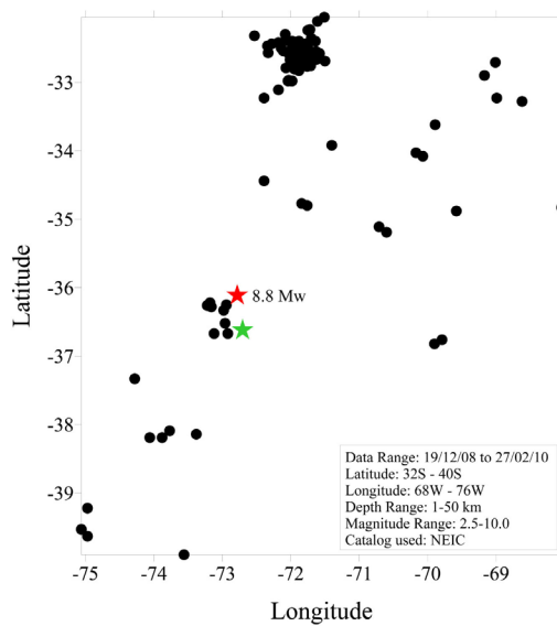
Figure 12. Chile earthquake of 27/02/2010 with the analyzed seismicity indicated with black circles. The location of the dynamic epicenter DEM 22 indicated with the green color star, while the red color star indicates the epicenter of the mainshock occurred.
