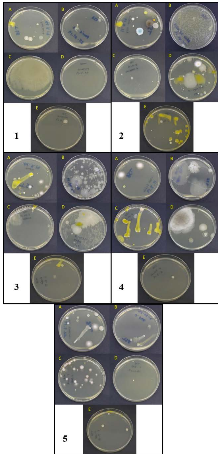
Figure 3. Bacterial growth at tryptic soy broth (TSB) medium on the sampling points of Poniente station (1), Arco Ladrillo station (2), La Rubia station (3), Vega Sicilia station (4) and Valladolid Sur station (5). (A) First sample; (B) second sample; (C) third sample; (D) fourth sample; (E) fifth sample.
