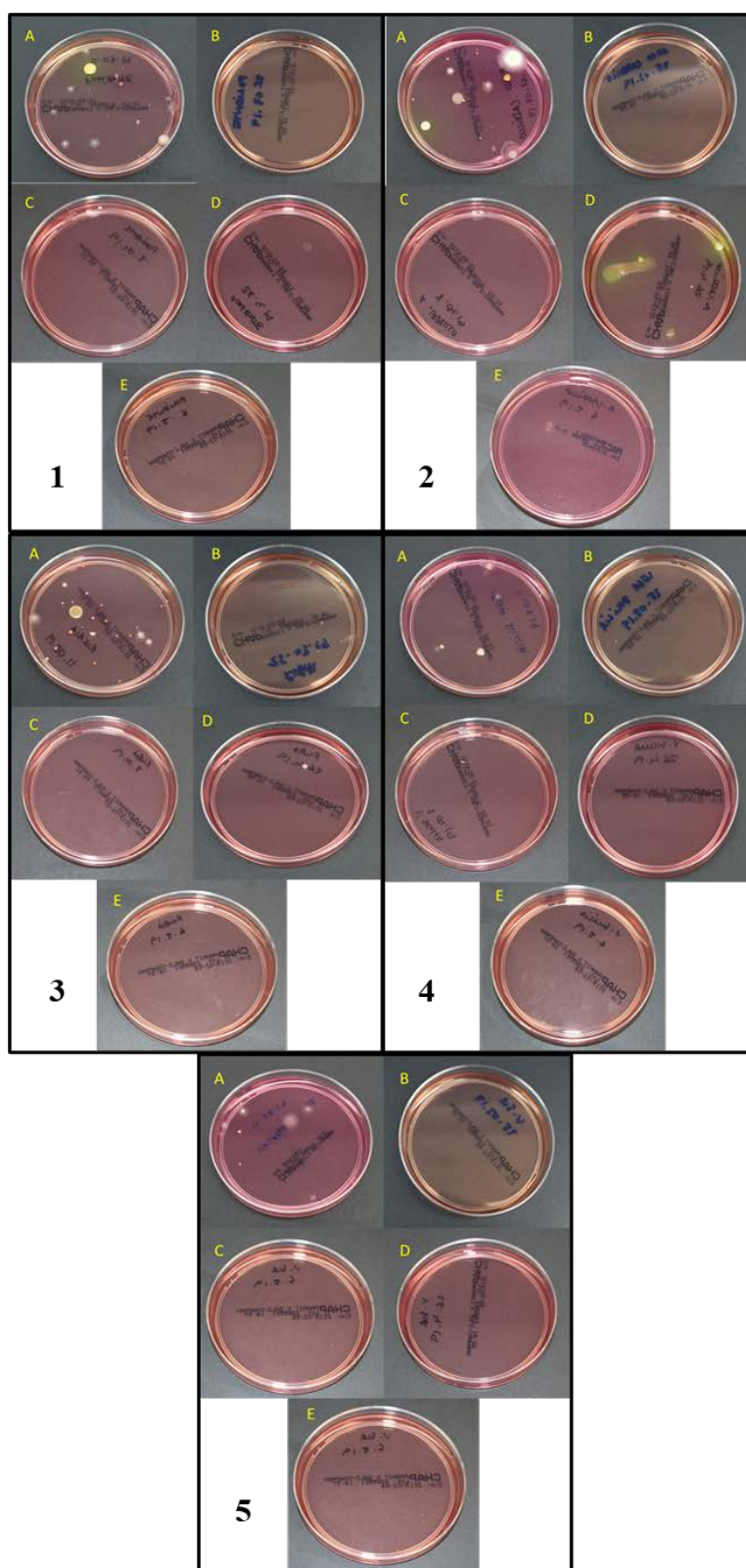
Figure 4. Bacterial growth at mannitol salt agar (Mannitol) medium on the sampling points of Poniente station (1), Arco Ladrillo station (2), La Rubia station (3), Vega Sicilia station (4) and Valladolid Sur station (5). (A) First sample; (B) second sample; (C) third sample; (D) fourth sample; (E) fifth sample.
