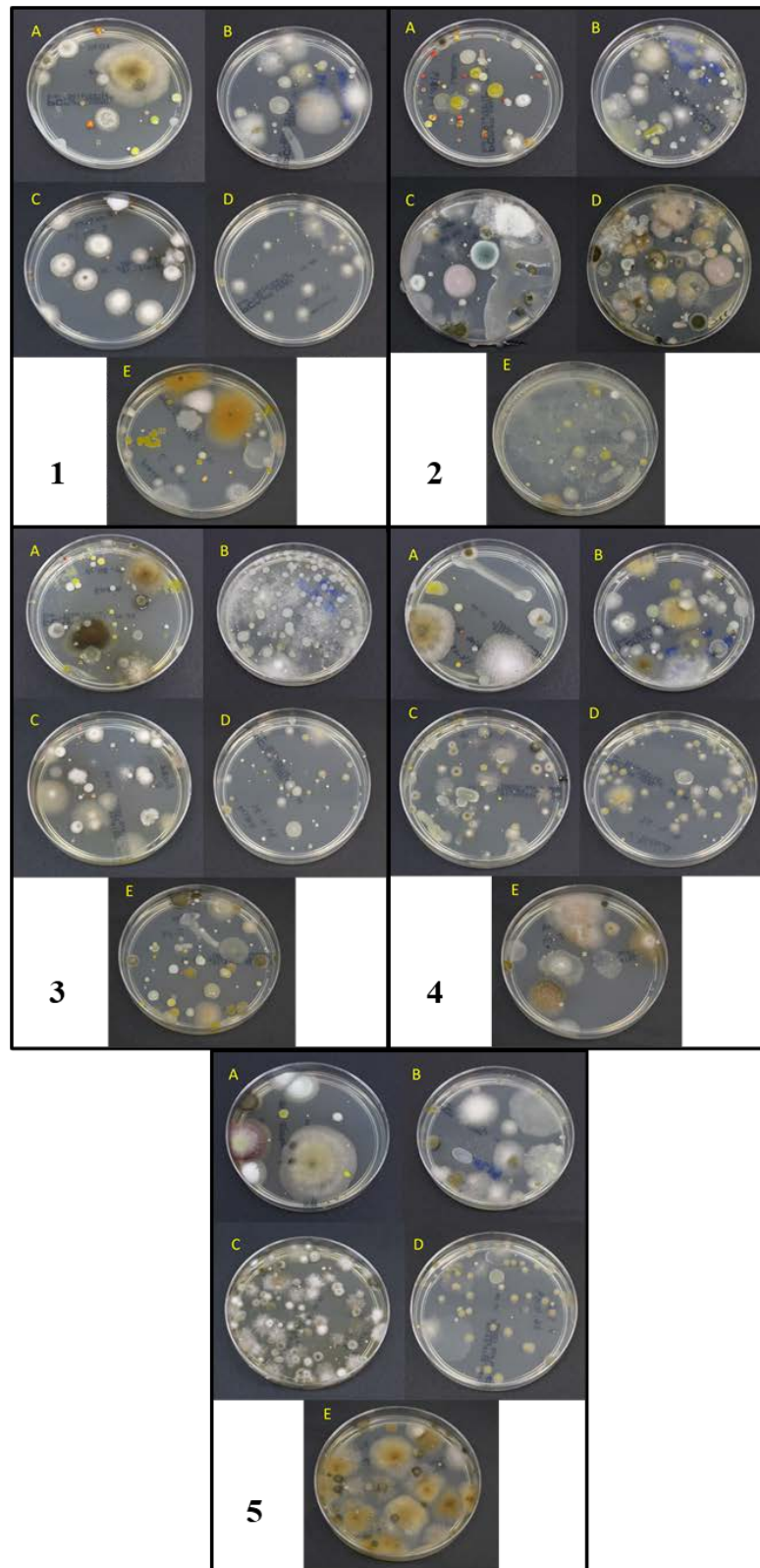
Figure 5. Bacterial growth at standard plate count agar (PC) medium on the sampling points of Poniente station (1), Arco Ladrillo station (2), La Rubia station (3), Vega Sicilia station (4) and Valladolid Sur station (5). (A) First sample; (B) second sample; (C) third sample; (D) fourth sample; (E) fifth sample.
