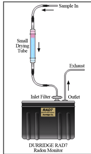
Figure 2. Schematic diagram for the Radon measurement in indoor air.
