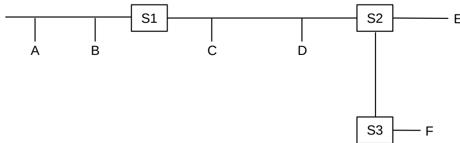
Fig. 13:: Ethernet with switches S1, S2 and S3
