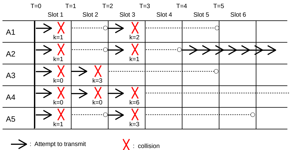
Fig. 11:: Ethernet collisions with exponential backoff
