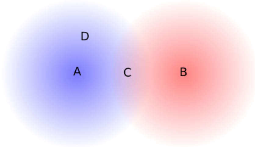
Fig. 23:: If A and B transmit simultaneously, there is a collision at C, reachable by both, but not at D
