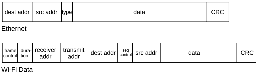
Fig. 26:: Top: Ethernet packet format; Bottom: Wi-Fi packet format (typical)
