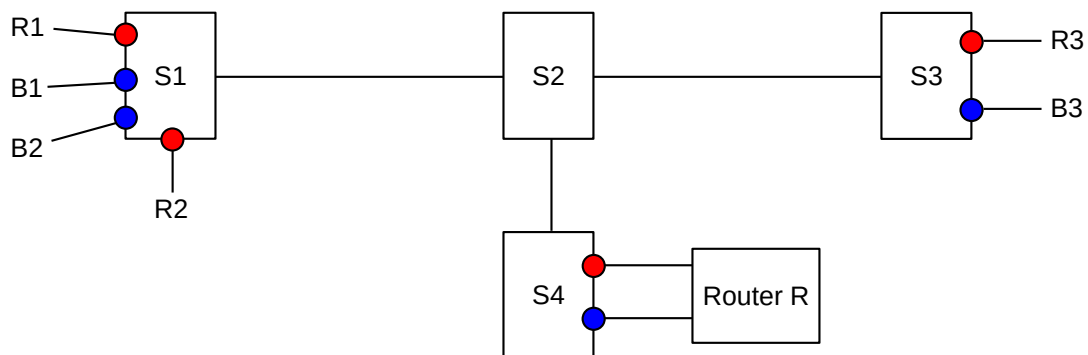
Fig. 16:: One network of switches S1-S4 divided into two VLANs, red and blue
