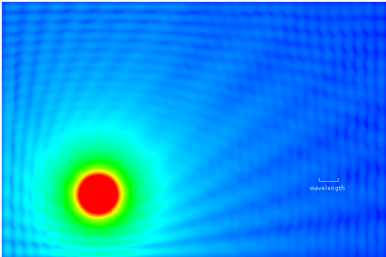
Fig. 22:: Signal-intensity map (simulated) in a room with walls with 40% reflectivity
