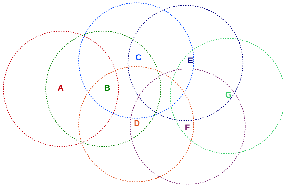
Fig. 28:: Typical MANET in which the radio range for each node is represented by a circle around that node. Node A can reach Node G either by the route A–B–C–D–G or by A–B–D–F–G (or by other routes)
