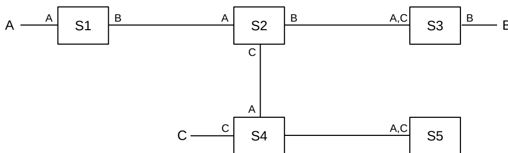
Fig. 14:: Five learning switches after three packet transmissions
