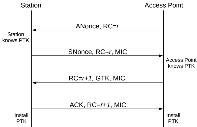
Fig. 27:: Four-way WPA2 handshake; RC represent the replay counter
