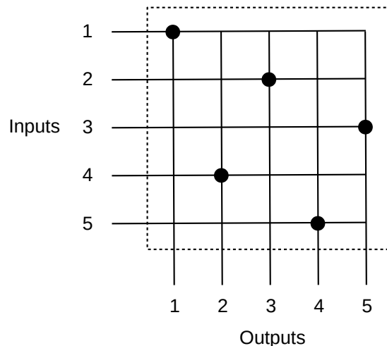
Fig. 17:: 5 \times 5 crossbar with 5 parallel connections 1 \rightarrow 1 , 2 \rightarrow 3 , 3 \rightarrow 5 , 4 \rightarrow 2 , 5 \rightarrow 4
