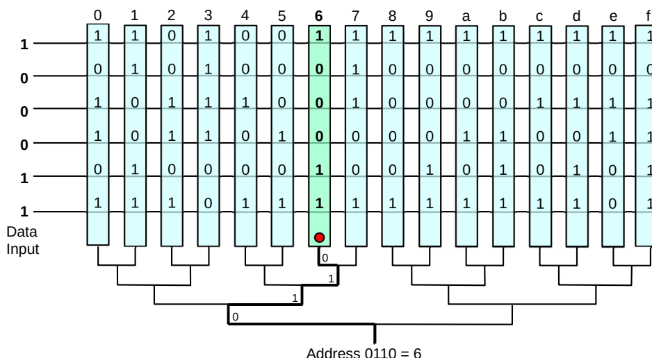
Fig. 18:: Content-Addressable Memory
