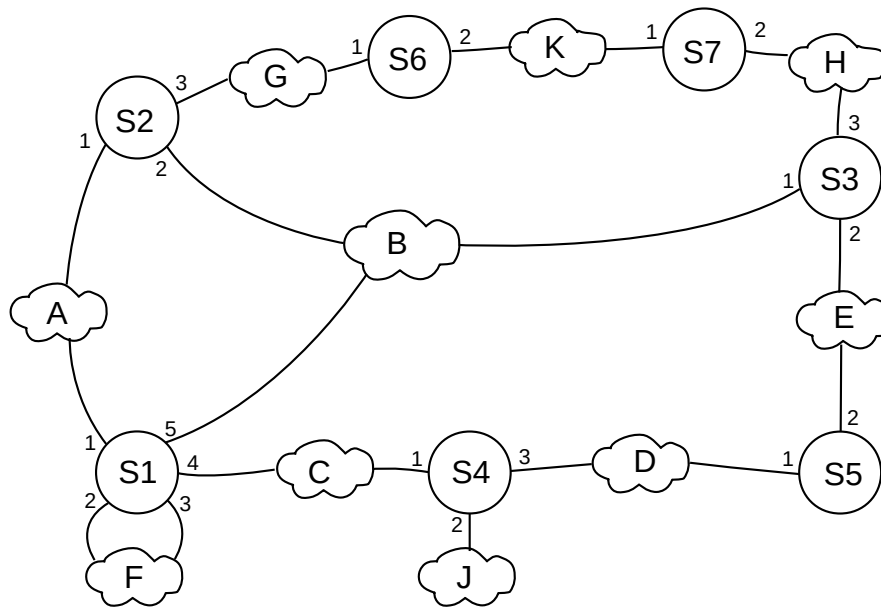
Fig. 15:: Switched Ethernet with potentially multiple hosts connected to switch ports
