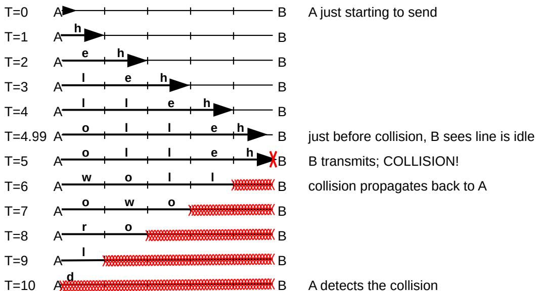
Fig. 10:: Ethernet collision, showing one full RTT before collision detectability
